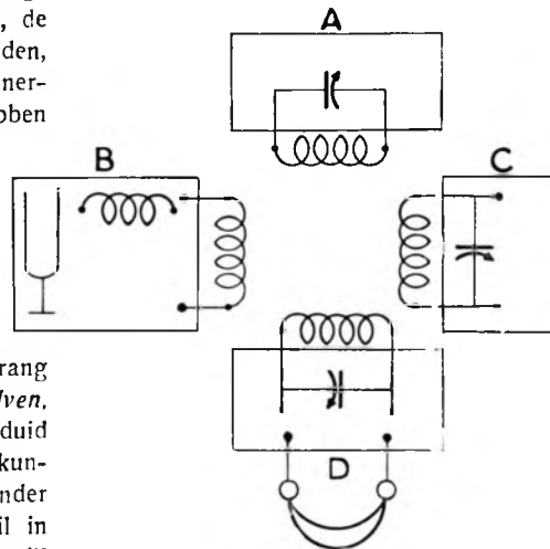
A = frequentie-meter. B = multivibrator. C = zwever. D = ontvanger.
